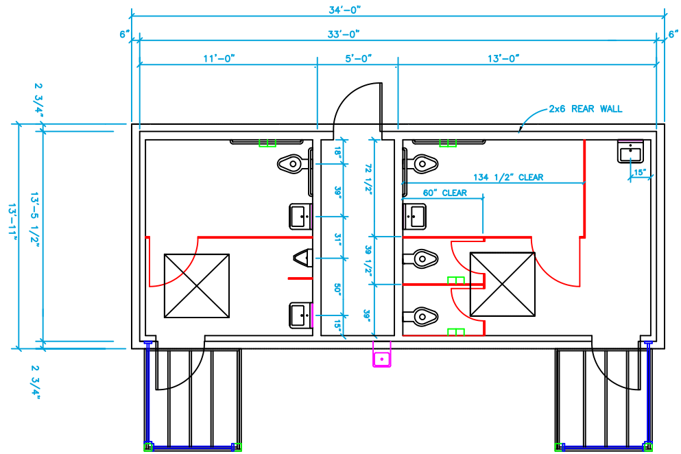
FLOOR PLAN
