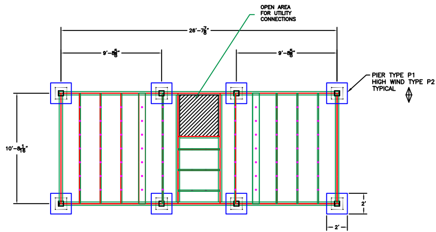
PIER LAYOUT
