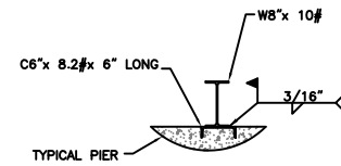
CONNECTION DETAIL @ PIER
