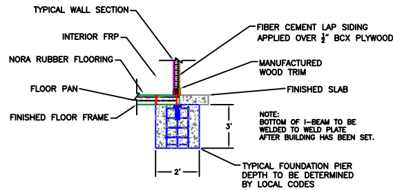
TYPICAL SECTION VIEW @ SUGGESTED PIER
