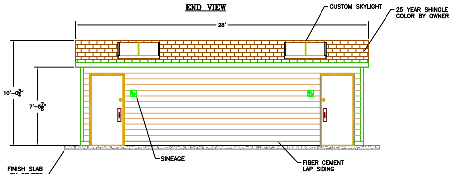
FRONT ELEVATION PRIVACY SCREENS NOT SHOWN
