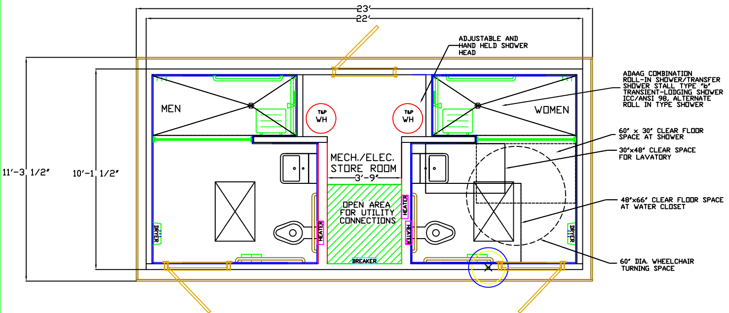
FLOOR PLAN
