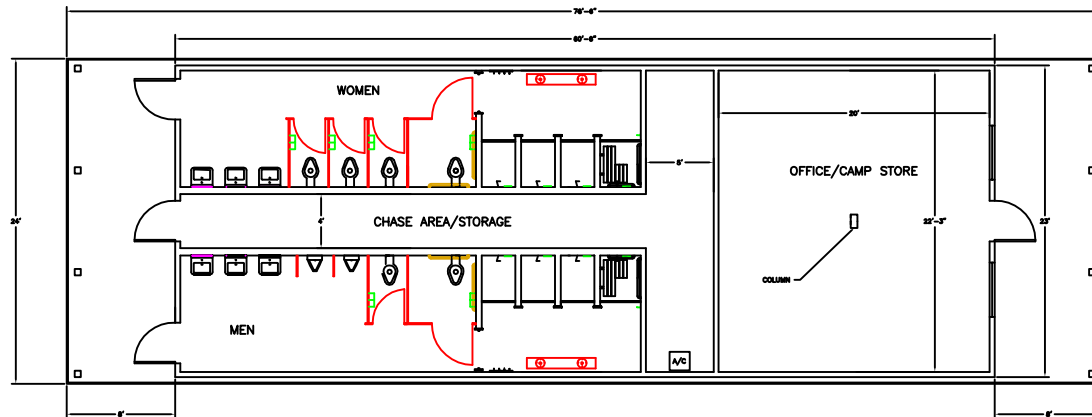
FLOOR PLAN
