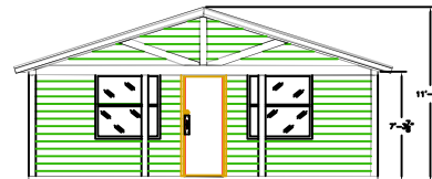
CAMP STORE/OFFICE END ELEVATION
