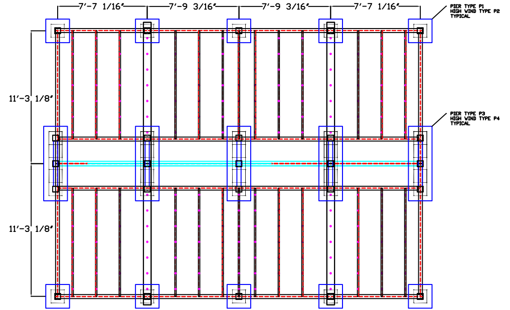
PIER LOCATION PLAN
