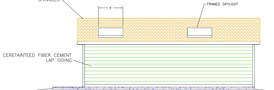
LEFT ELEVATION PRIVACY SCREEN NOT SHOWN
