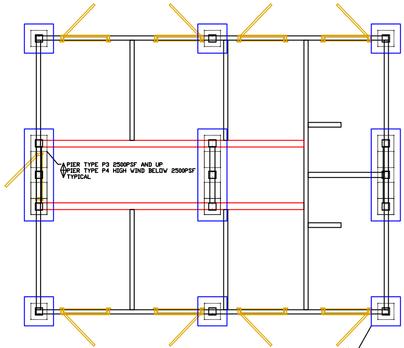
PIER PLAN
