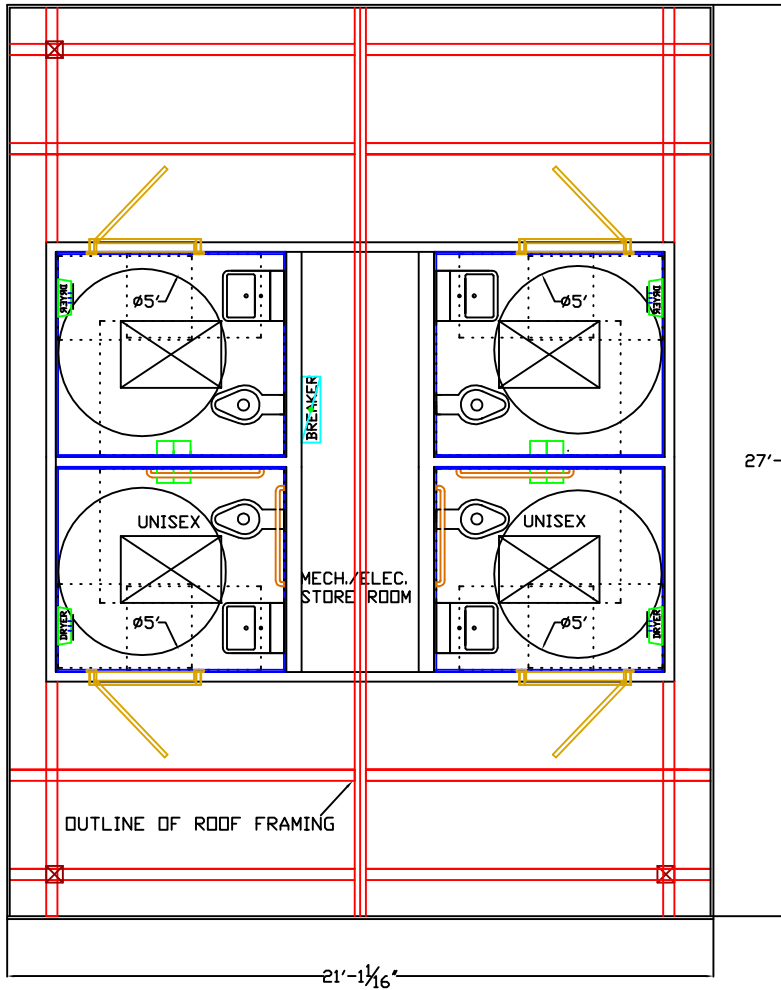
FLOOR PLAN
